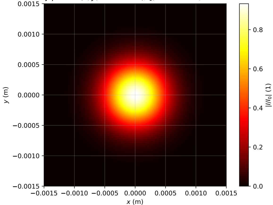
Intensity profile I(x, y, z = 0.637m)/I_0 , Pin=0.1Pcr, artificial time
